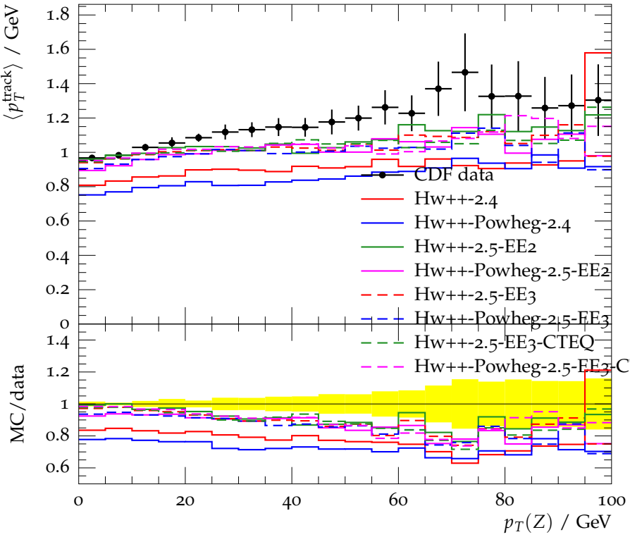
Transverse region charged p_{\perp} average
