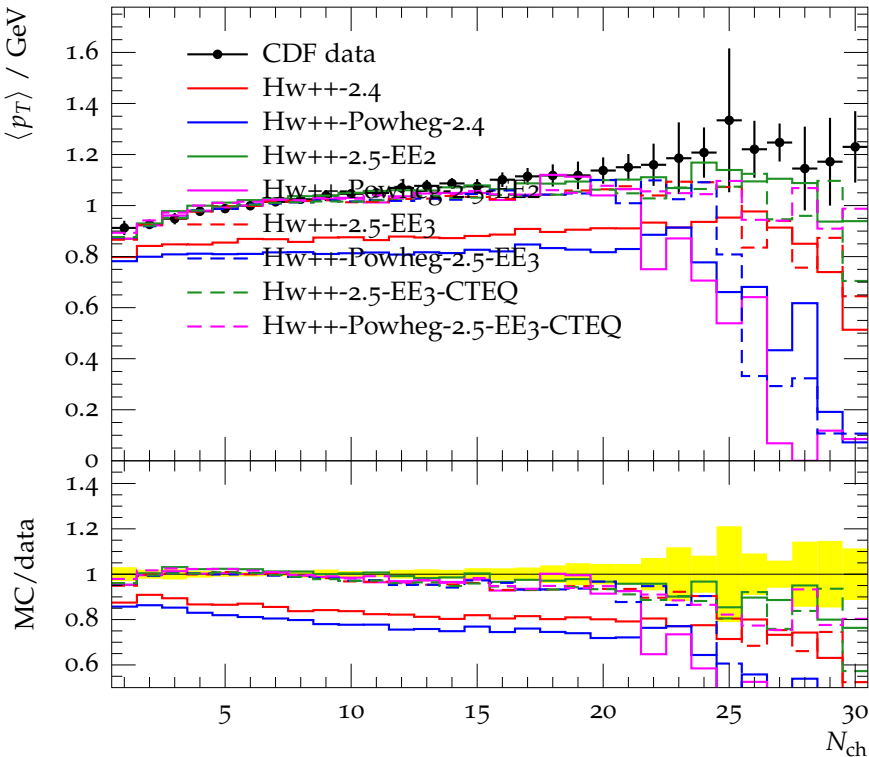
Average charged p_{\perp} vs charged multiplicity, p_{\perp}(Z) less than 10 GeV
