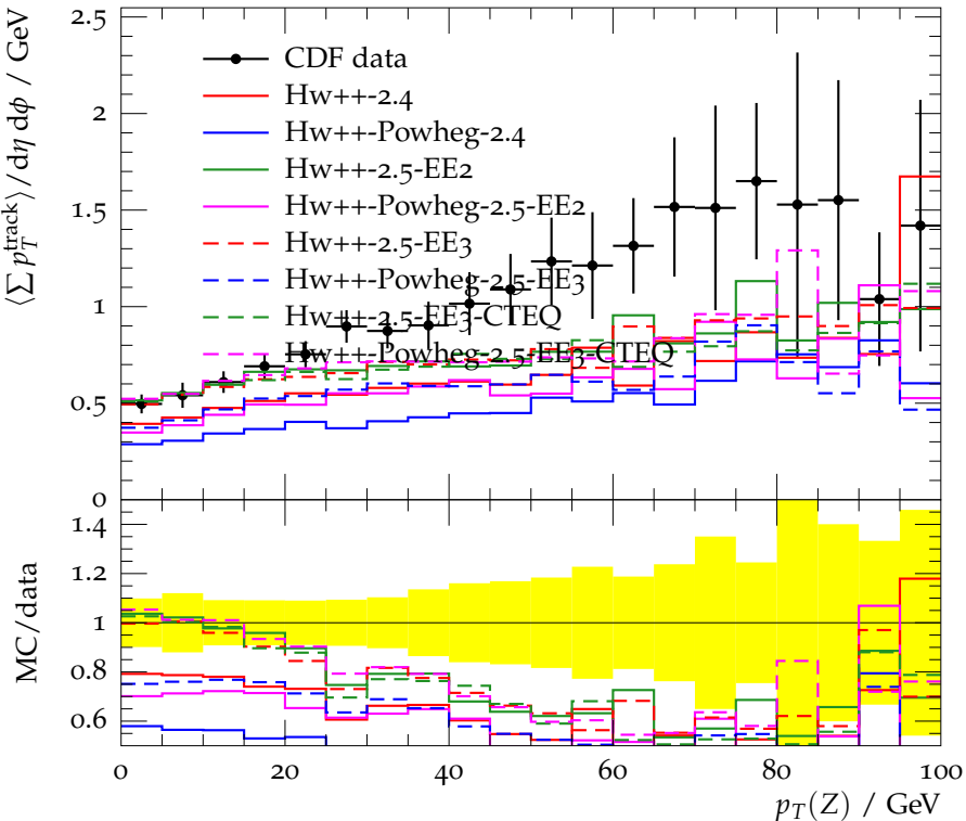
TransDIF region charged p_{\perp}^{\text{sum}} density
