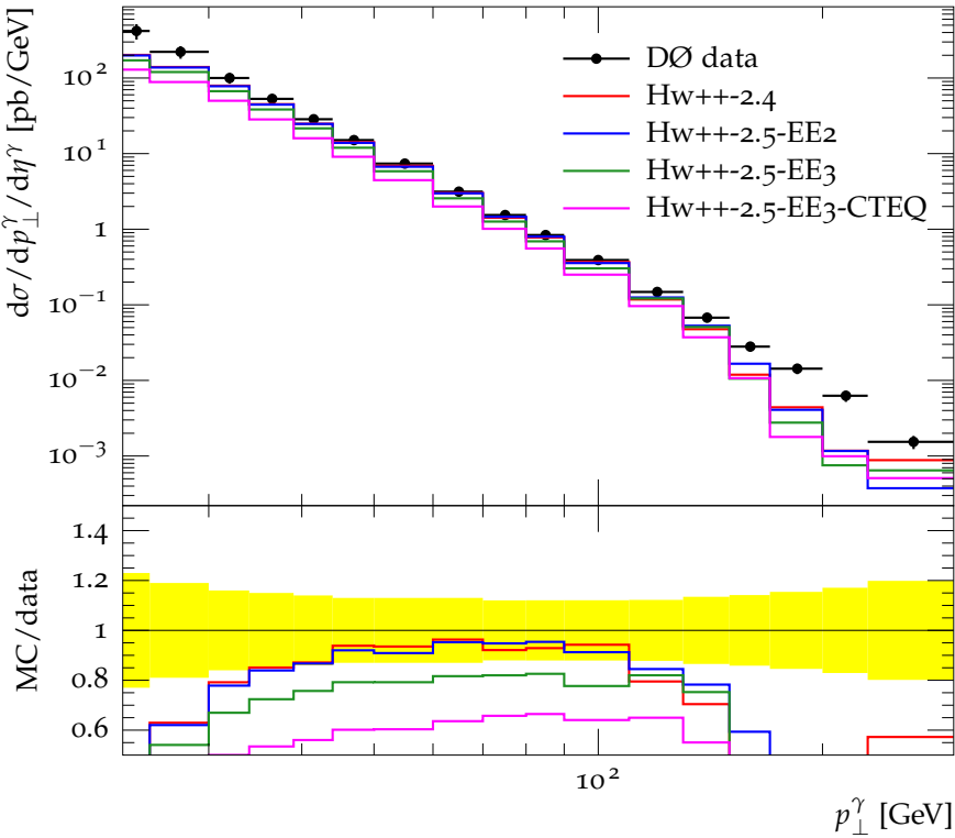
p_{\perp} spectrum for leading photon
