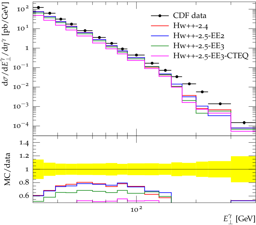
Transverse energy of isolated prompt photon
