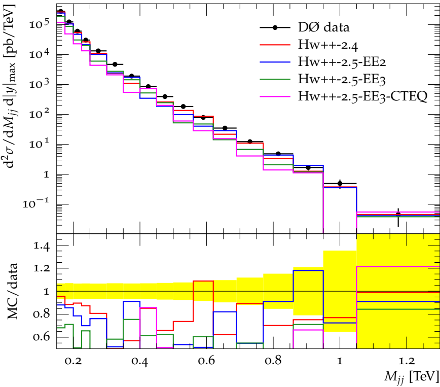
Dijet invariant mass for |y|_{\max} < 0.4
