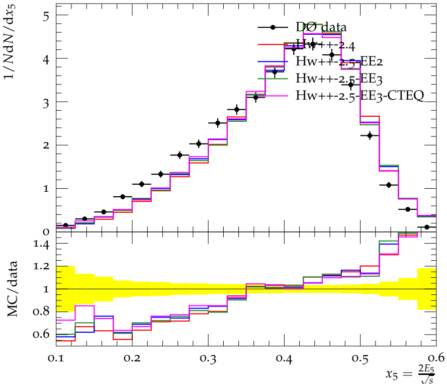
Energy fraction of 3rd jet in 4-jet events
