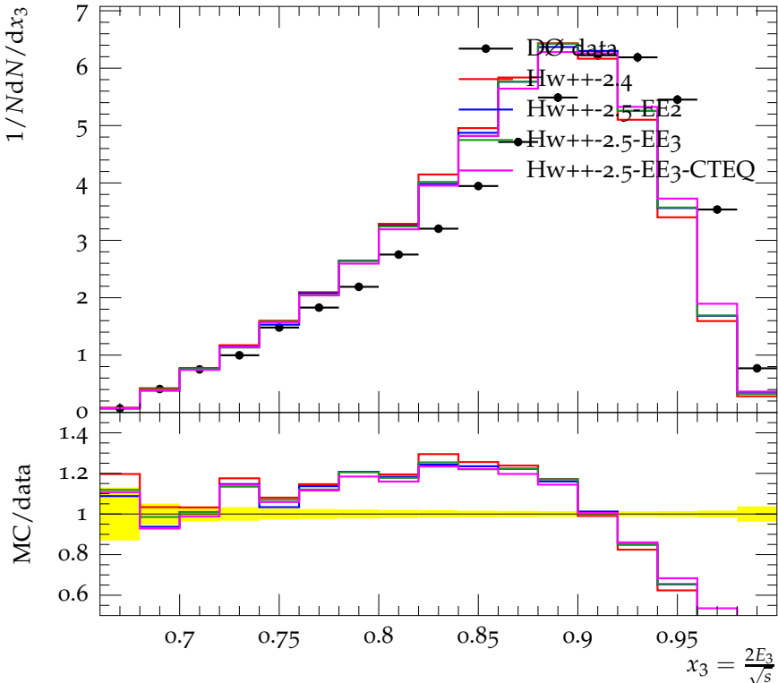
Energy fraction of hardest jet in 3-jet events
