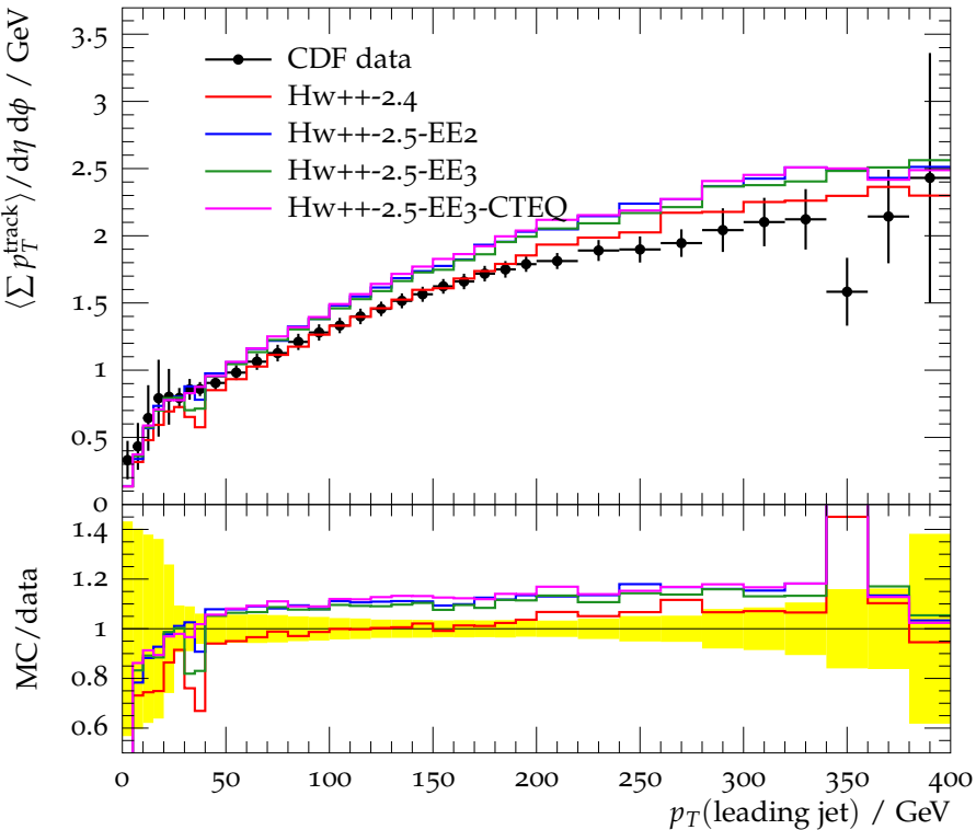
TransDIF region charged \Sigma p_{\perp} density
