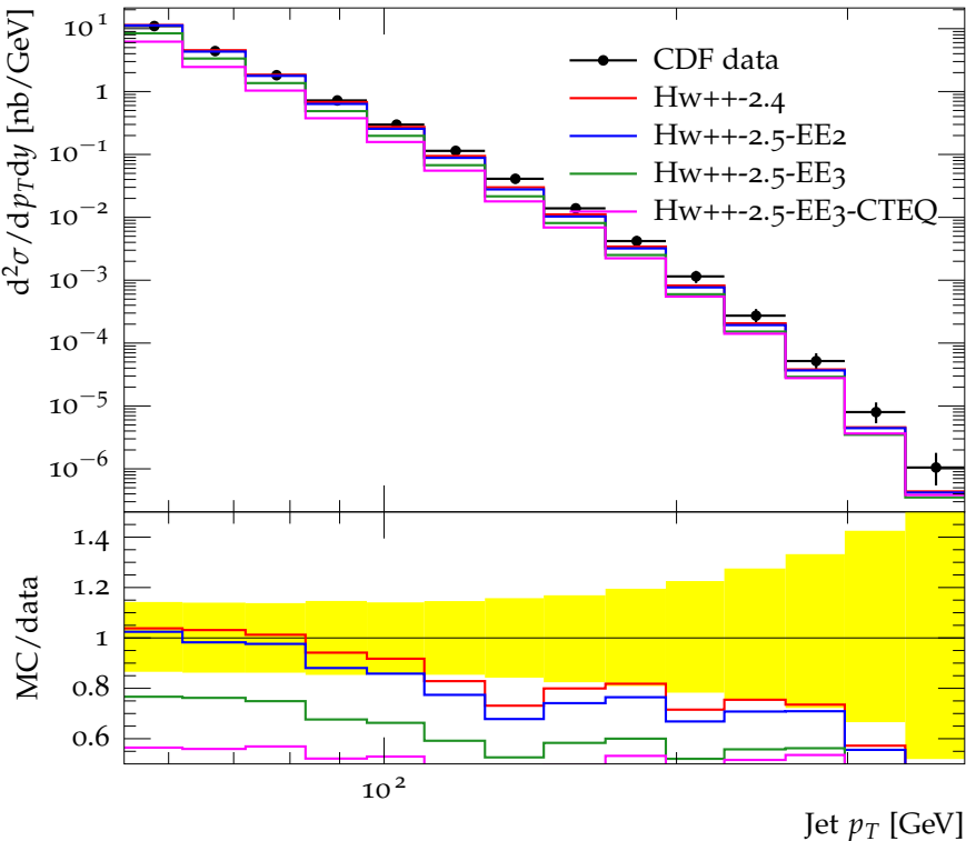
Inclusive jet cross-section vs p_T for 1.1 < |\eta| < 1.6, D = 0.7
