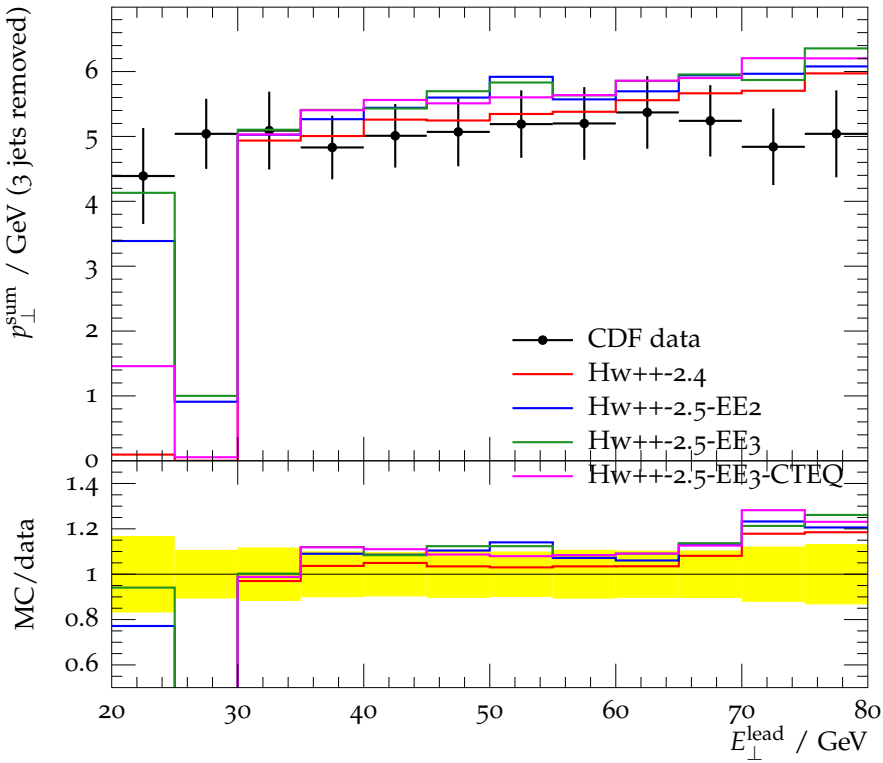
Swiss Cheese p_{\perp}^{\text{sum}} vs. E_{\perp}^{\text{lead}} (3 jets removed) at \sqrt{s} = 630 GeV
