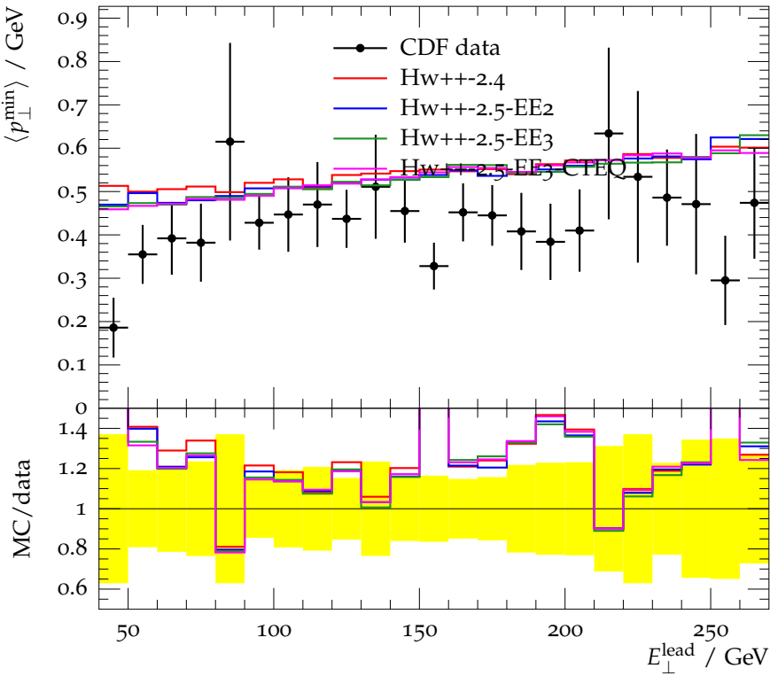
Transverse cone \langle p_{\perp}^{\min} \rangle vs. E_{\perp}^{\text{lead}} at \sqrt{s} = 1800 GeV
