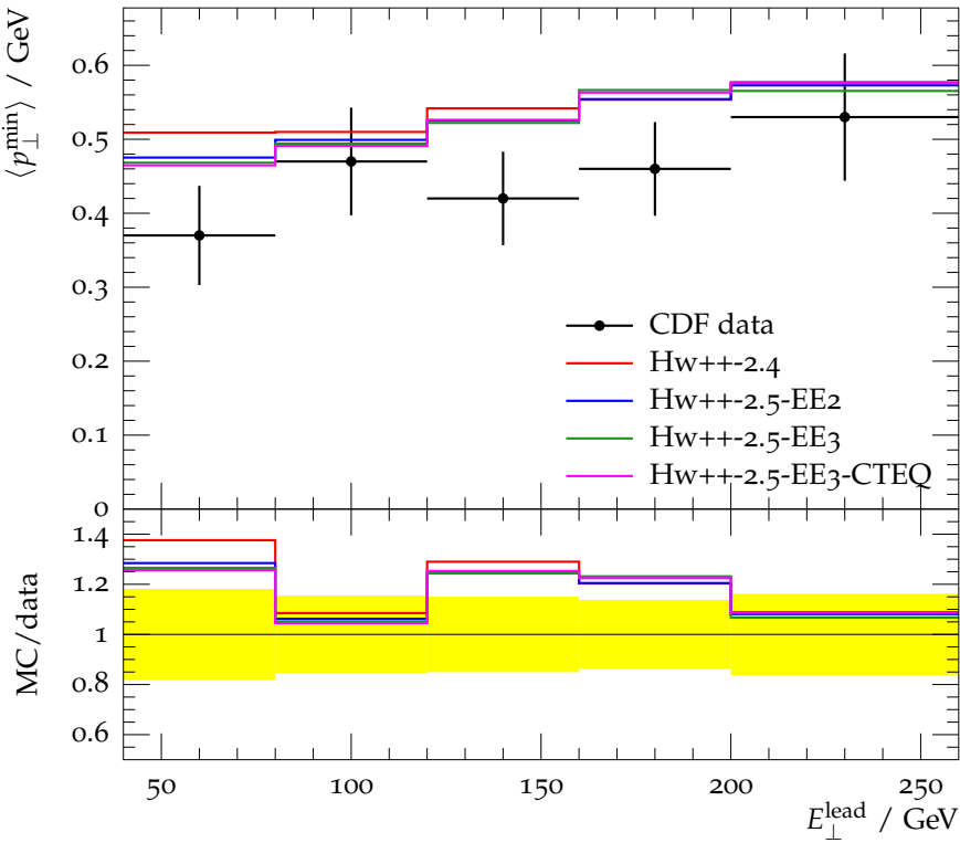
Transverse cone \langle\langle p_{\perp}^{\min}\rangle\rangle vs. E_{\perp}^{\text{lead}} at \sqrt{s} = 1800 GeV
