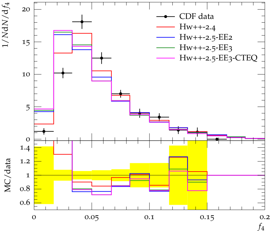
Single-jet mass fraction in inclusive 3-jet events
