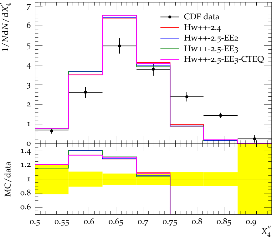
Dalitz distribution in inclusive 5-jet events
