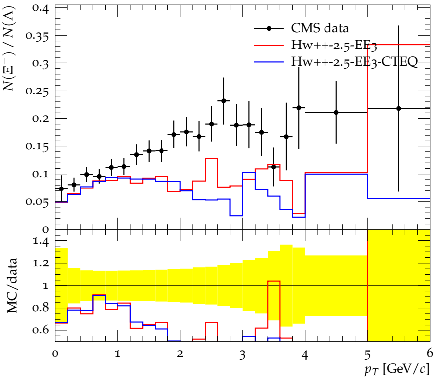
E^- / \Lambda versus transverse momentum at \sqrt{s} = 0.9 TeV
