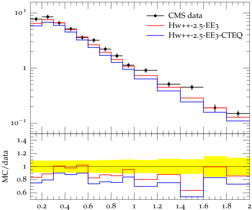
Charged hadron p_{\perp} for |\eta| = 1.5 at \sqrt{s} = 2.36 TeV
