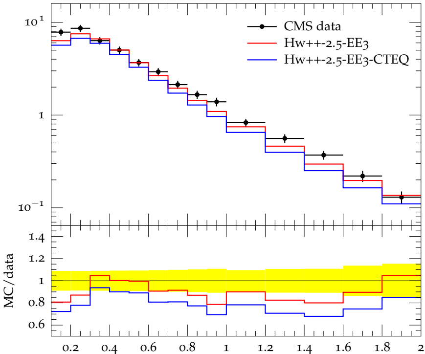
Charged hadron p_{\perp} for |\eta| = 1.3 at \sqrt{s} = 2.36 TeV
