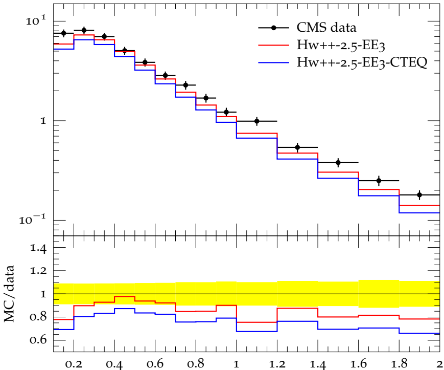
Charged hadron p_{\perp} for |\eta| = 0.9 at \sqrt{s} = 2.36 TeV
