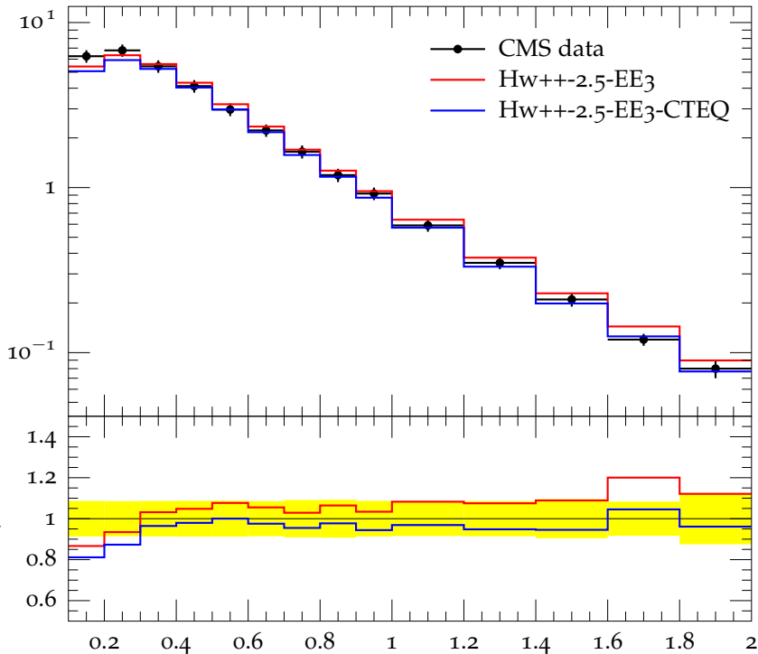
Charged hadron p_{\perp} for |\eta| = 1.3 at \sqrt{s} = 0.9 TeV
