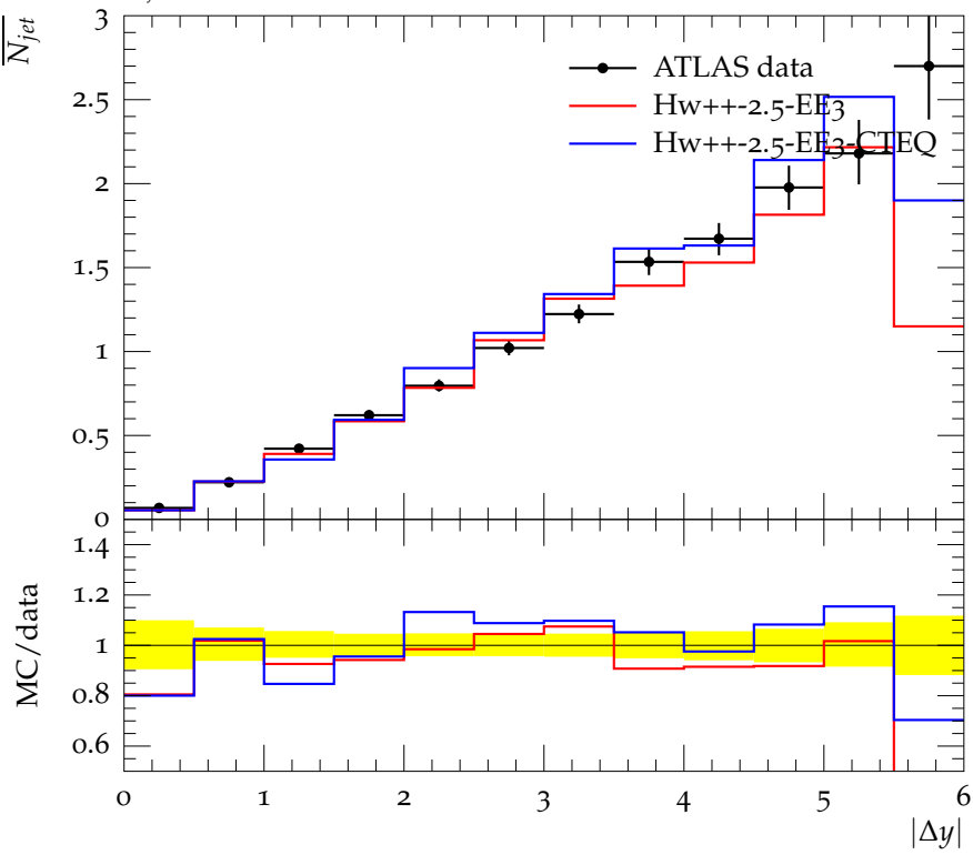
\overline{N}_{jet} vs |\Delta y| for 150 < \overline{P}_T < 180 , Fwd/Bwd
