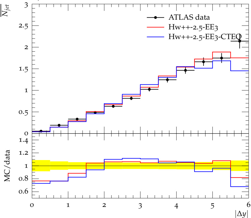
\overline{N}_{jet} vs |\Delta y| for 90 < \overline{P}_T < 120 , Fwd/Bwd
