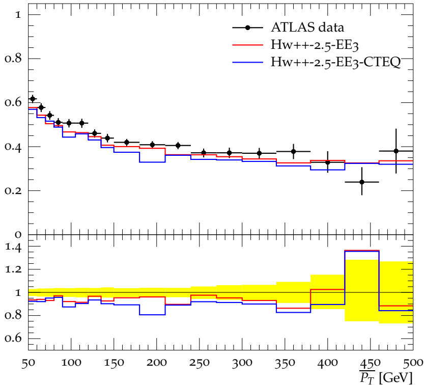
Gap fraction vs \overline{P_T} for 2.0 < |\Delta y| < 3.0 , Fwd/Bwd
