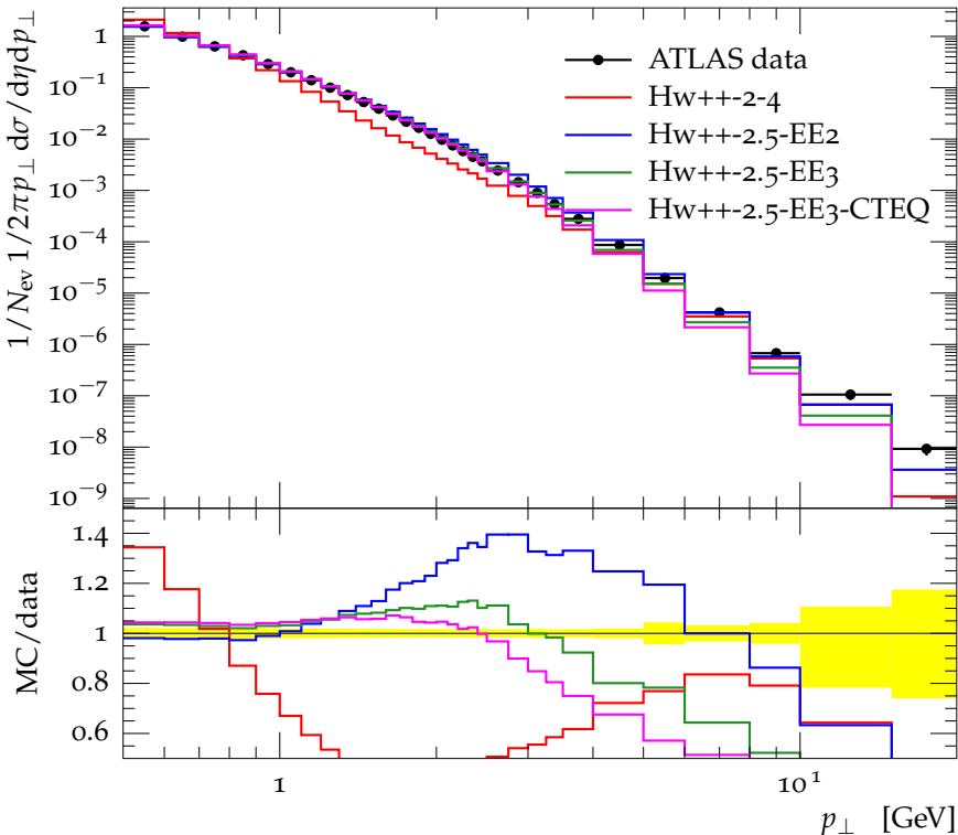
Charged particle p_{\perp} at 900 GeV, track p_{\perp} > 500 MeV, for N_{\text{ch}} \geq 6
