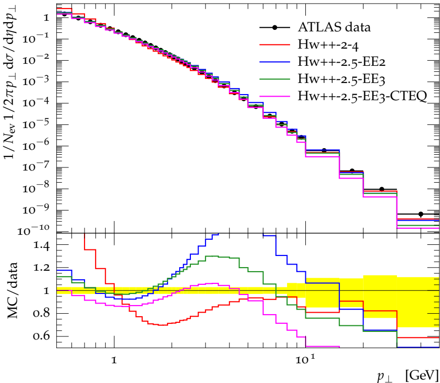
Charged particle p_{\perp} at 7 TeV, track p_{\perp} > 500 MeV, for N_{\text{ch}} \geq 1
