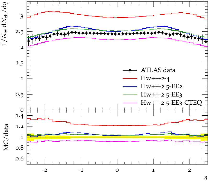
Charged particle \eta at 7 TeV, track p_{\perp} > 500 MeV, for N_{\text{ch}} \geq 1
