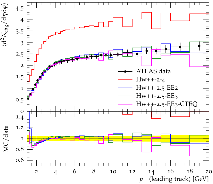
Away N_{\text{chg}} density vs. p_{\perp}^{\text{trk1}} , \sqrt{s} = 7 TeV, p_{\perp} > 100 MeV
