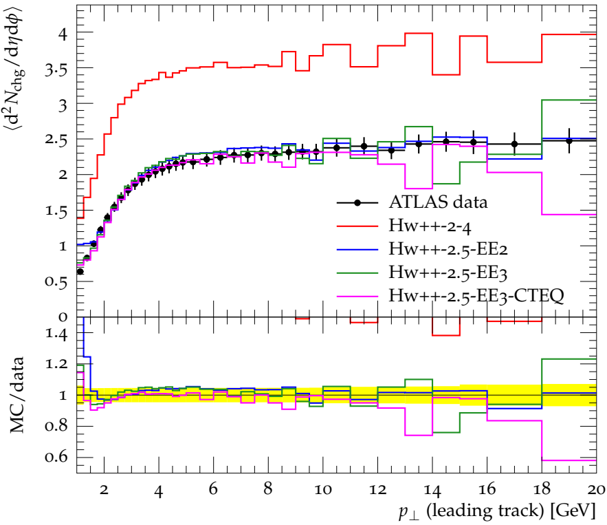
Toward N_{\text{chg}} density vs. p_{\perp}^{\text{trk1}} , \sqrt{s} = 7 TeV, p_{\perp} > 100 MeV
