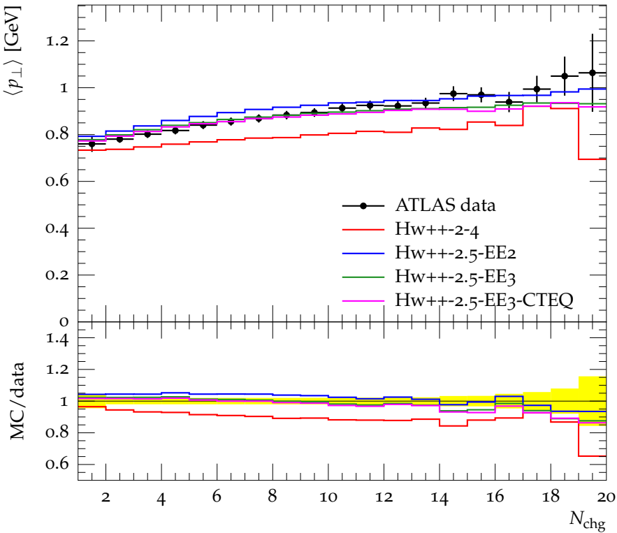
Away \langle p_{\perp} \rangle vs. N_{\text{chg}} , \sqrt{s} = 900 GeV
