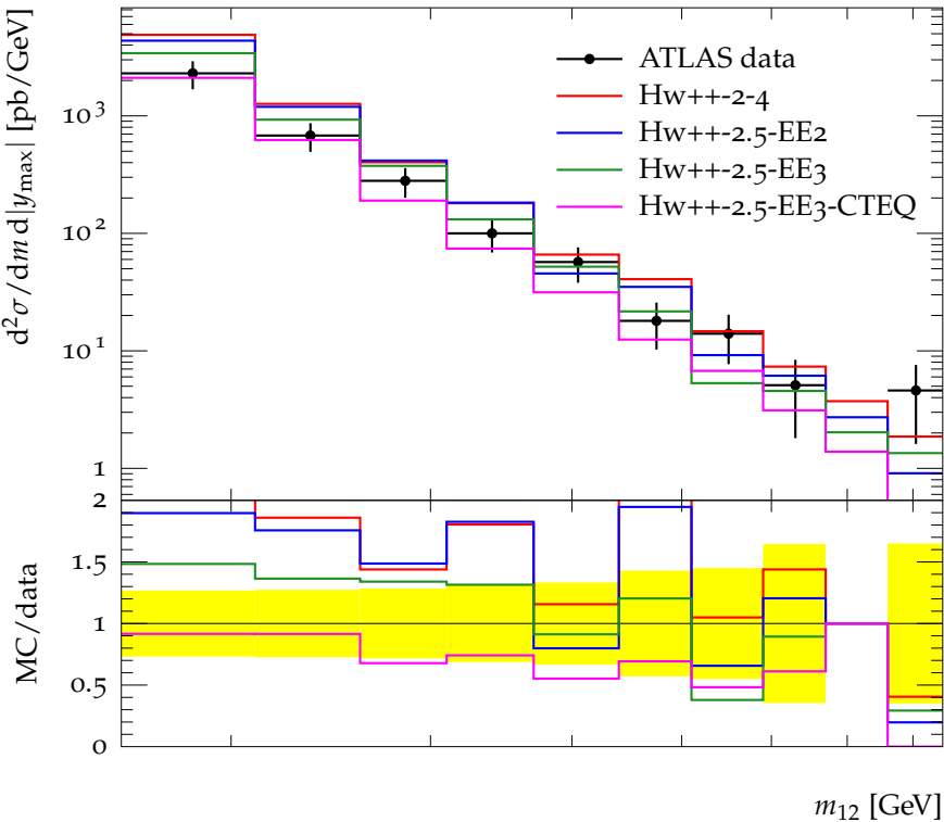
Dijet mass spectrum for 0.3 < |y_{\max}| < 0.8 . anti-KT, R = 0.4 .
