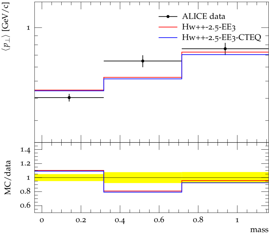
Average p_{\perp} vs mass, |\eta| < 0.5 , \sqrt{s} = 0.9 TeV (INEL)
