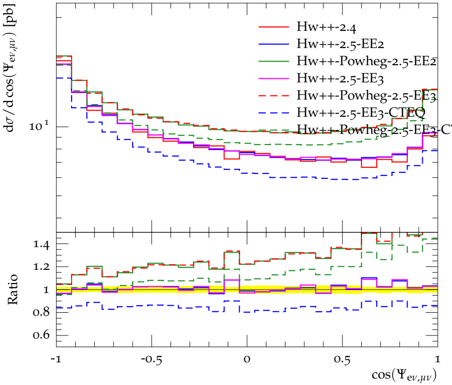
Angle between the boson decay planes
