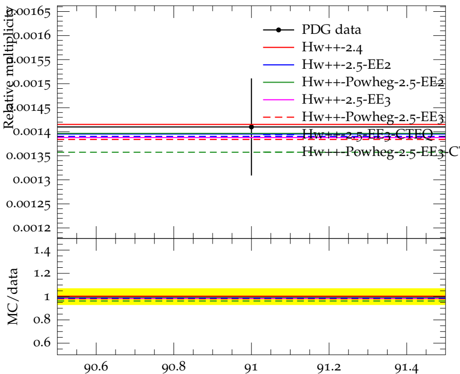
Ratio (w.r.t. \pi^\pm ) of mean \Sigma^-(1385) multiplicity
