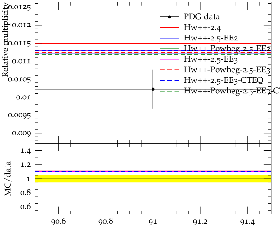
Ratio (w.r.t. \pi^\pm ) of mean \Sigma^\pm multiplicity
