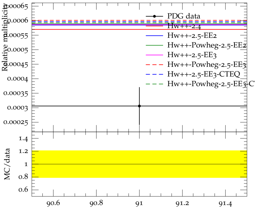
Ratio (w.r.t. \pi^\pm ) of mean D_{s1}^+ multiplicity
