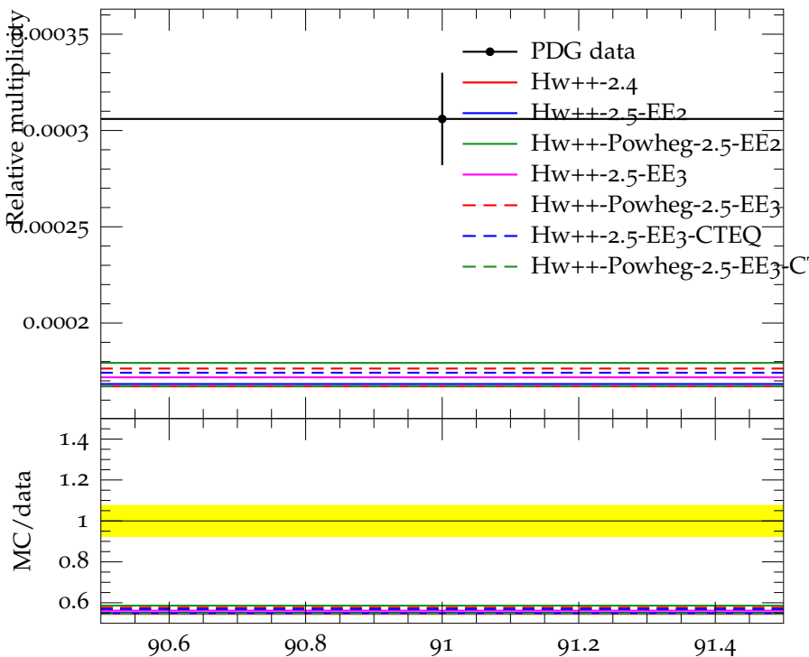
Ratio (w.r.t. \pi^\pm ) of mean J/\psi(1S) multiplicity
