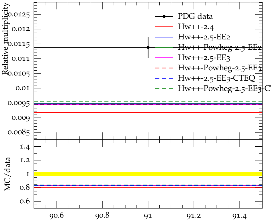
Ratio (w.r.t. \pi^\pm ) of mean D^{*+} (2010) multiplicity
