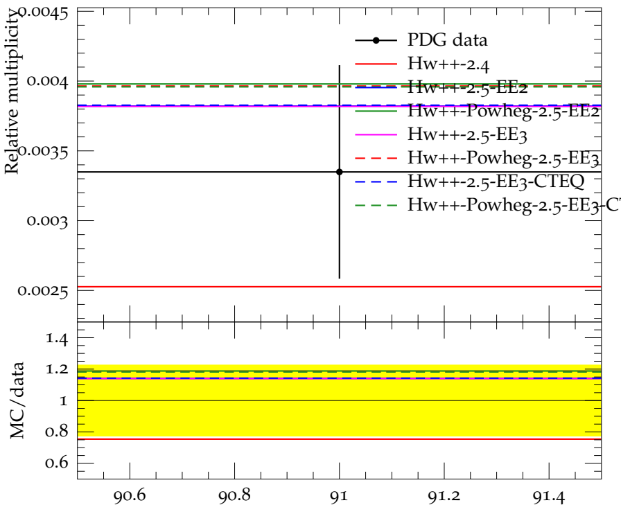
Ratio (w.r.t. \pi^\pm ) of mean B_s^0 multiplicity
