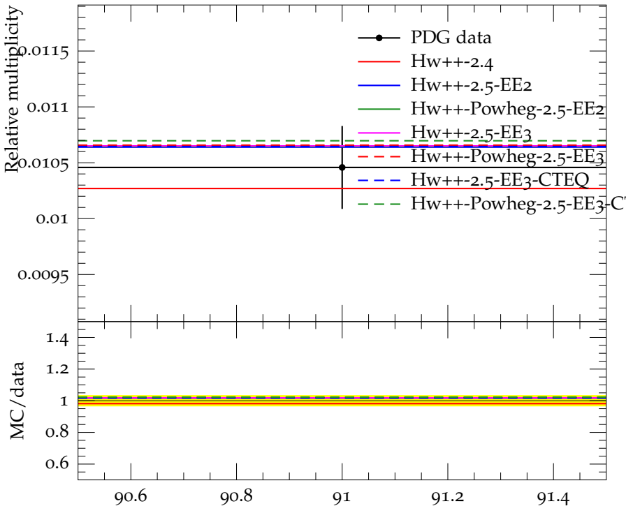
Ratio (w.r.t. \pi^\pm ) of mean B_u^+ multiplicity
