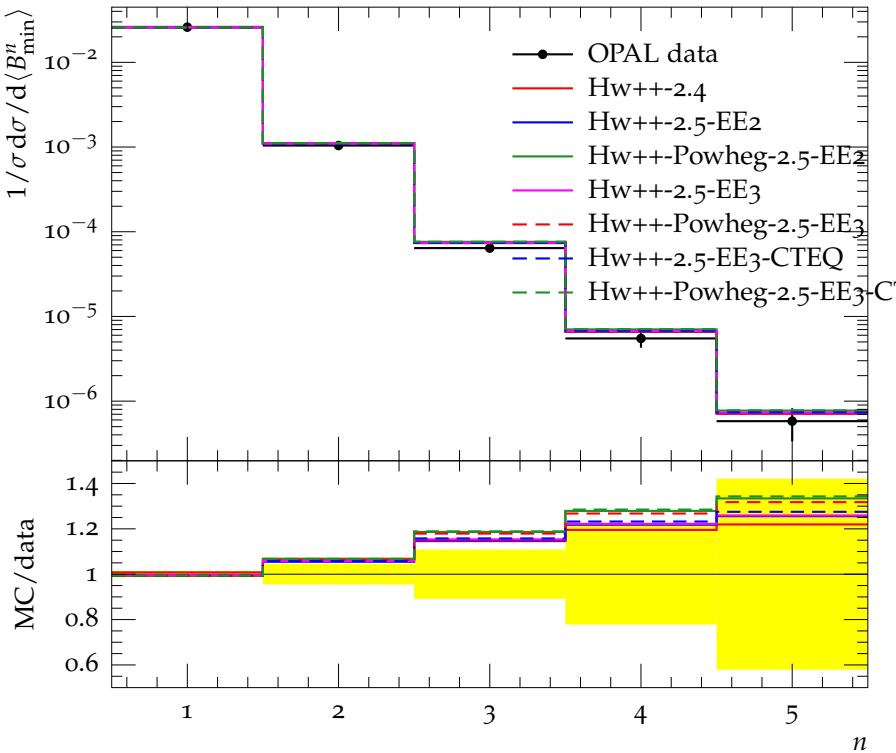
Moments of B_{\min} at 197 (189–209) GeV
