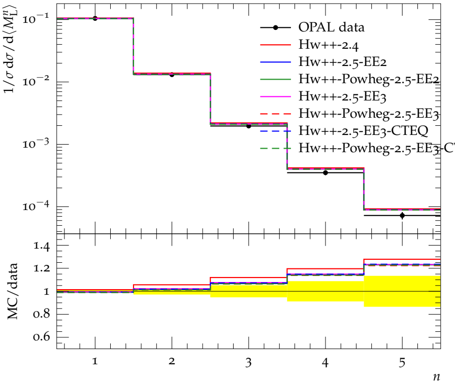
Moments of M_L at 197 (189–209) GeV
