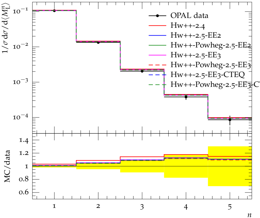
Moments of M_L at 177 (161–183) GeV
