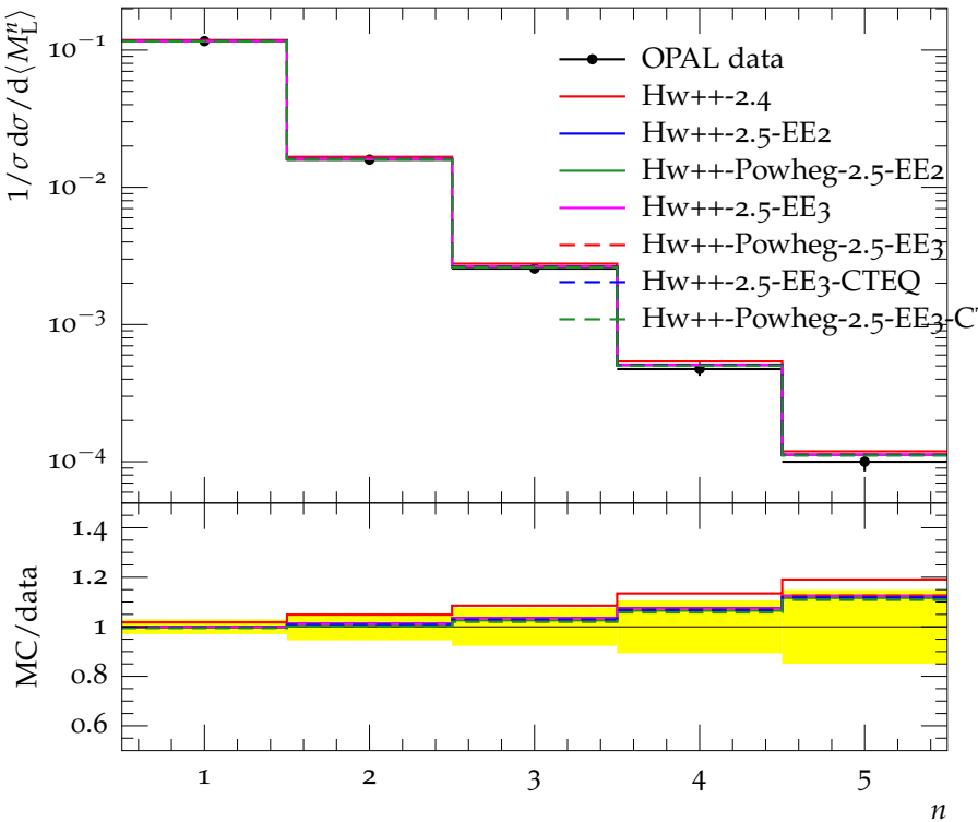
Moments of M_L at 133 GeV
