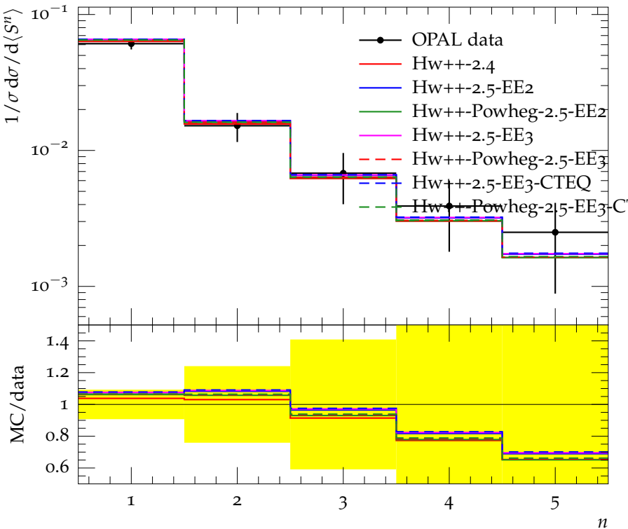
Moments of S at 177 (161–183) GeV
