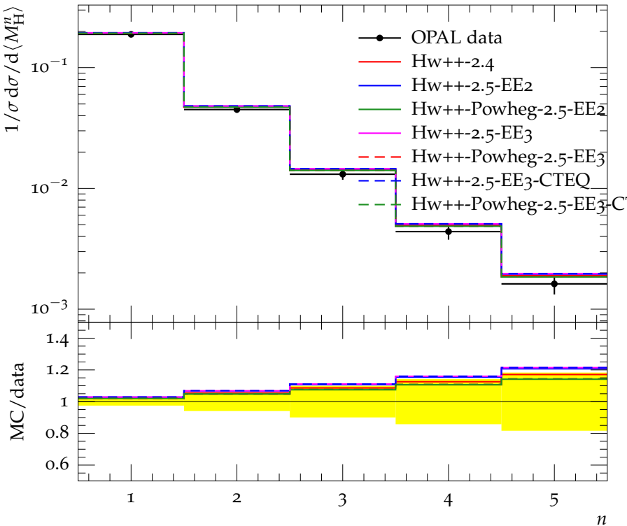
Moments of M_H at 177 (161–183) GeV
