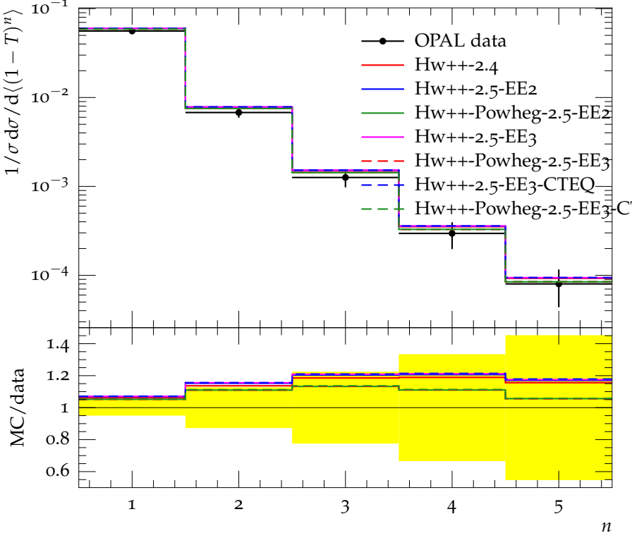
Moments of 1 - T at 177 (161–183) GeV
