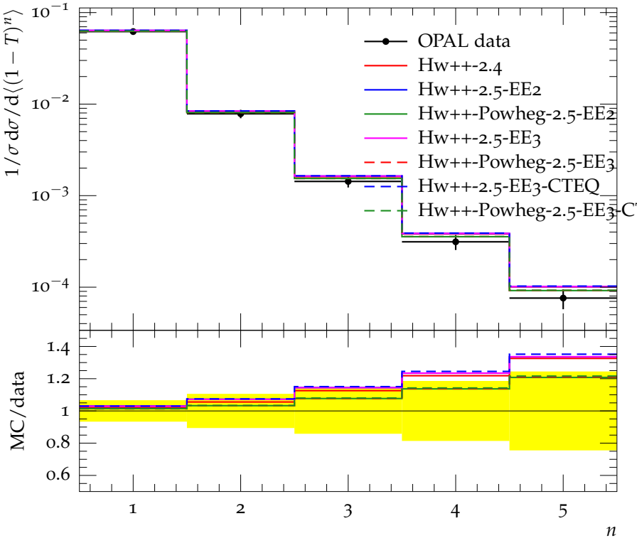
Moments of 1 - T at 133 GeV
