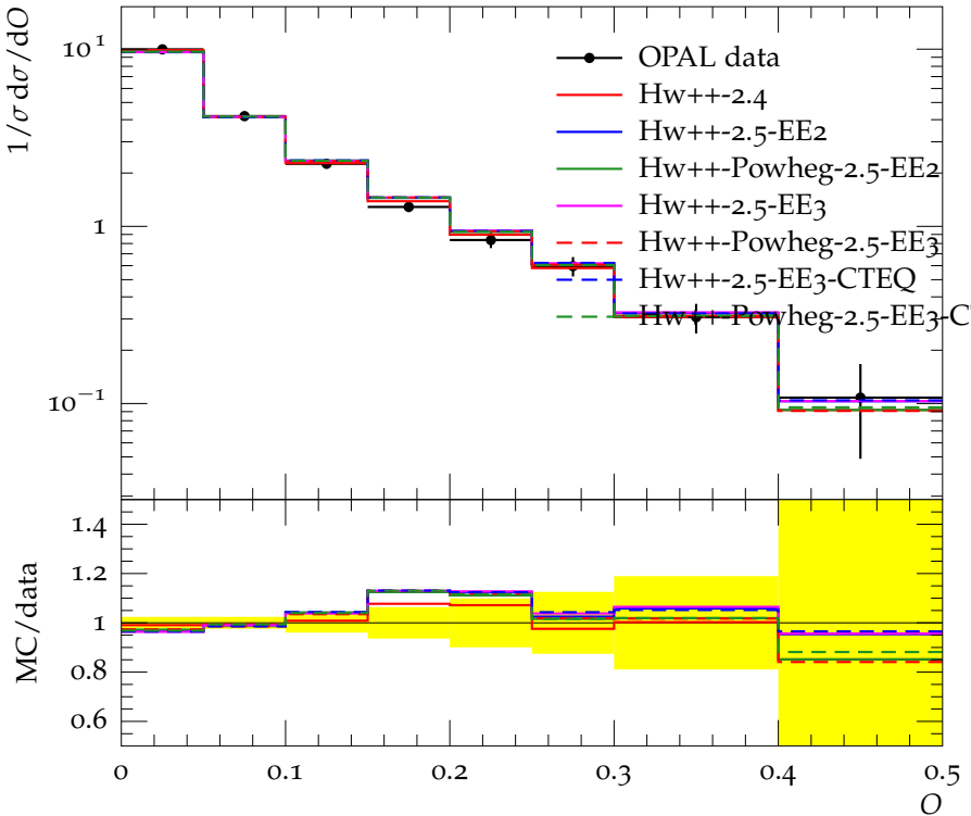
Oblateness, O , at 197 (189–209) GeV
