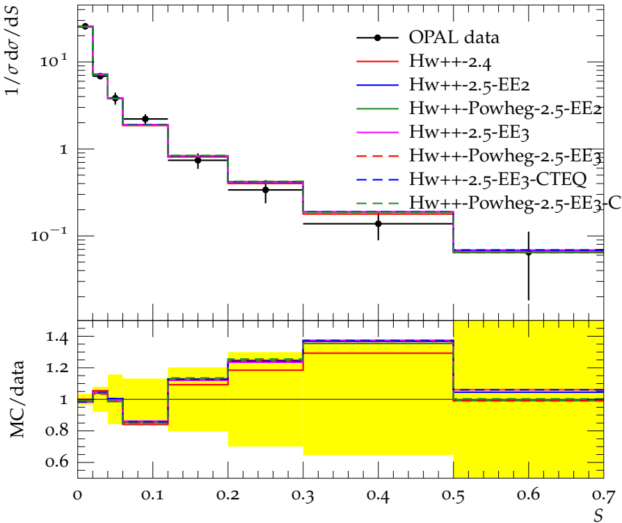
Sphericity, S , at 177 (161–183) GeV
