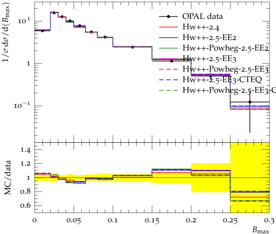
Wide hemisphere broadening, B_{\max} , at 197 (189–209) GeV
